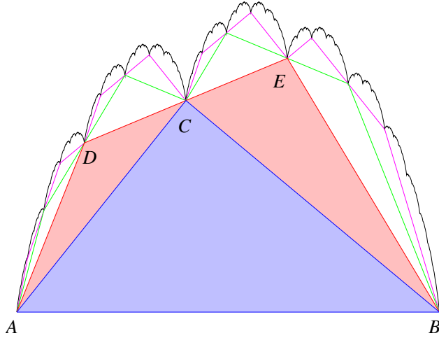
FIGURE 4: The first four steps in the construction of f_p^\omega , for p = 0.4 . In the first step, we transform the original interval AB into the polygonal line ACB , where C = \alpha_p^L(B) = \alpha_p^R(A) . In the second step, we similarly map the segment AC onto the segments AD and DC , and the segment CB onto CE and EB , by applying the same affine transformations. The procedure is then iterated yielding an increasing sequence of piecewise-linear functions, converging to the self-affine function f_p^\omega .
