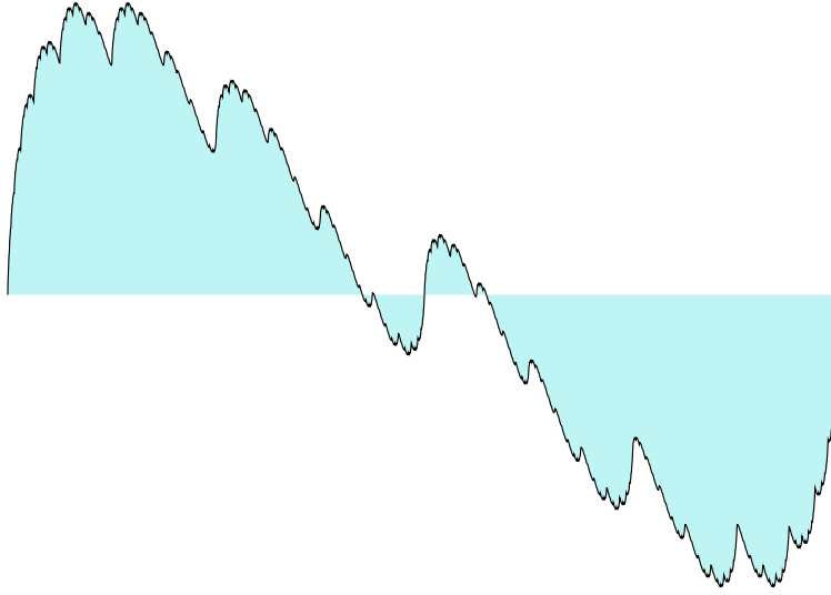
FIGURE 7: The limiting curve corresponding to the array \nabla'_{1/2} , obtained along the sequence (2k, k) . Notice that this curve does not have the same self-similarity as \ell^{\setminus p} , and is thus much less stable. For example, along the sequence (2k - 1, k - 1) the limiting curve is the left half, which is different.
